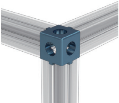
3-WAY EXTRUSION END CONNECTOR WITH PANEL CUTOUTS
